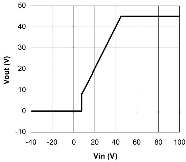
Figure 6 – Output Voltage vs Input Voltage
