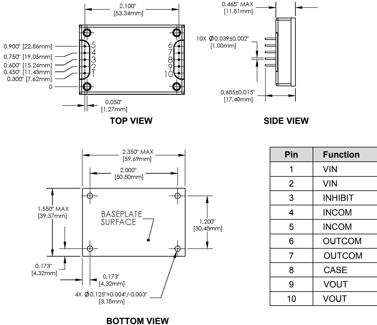
Figure 13 – Package and Pinout (Dimensional Limits are \pm 0.005 " Unless Otherwise Stated)
